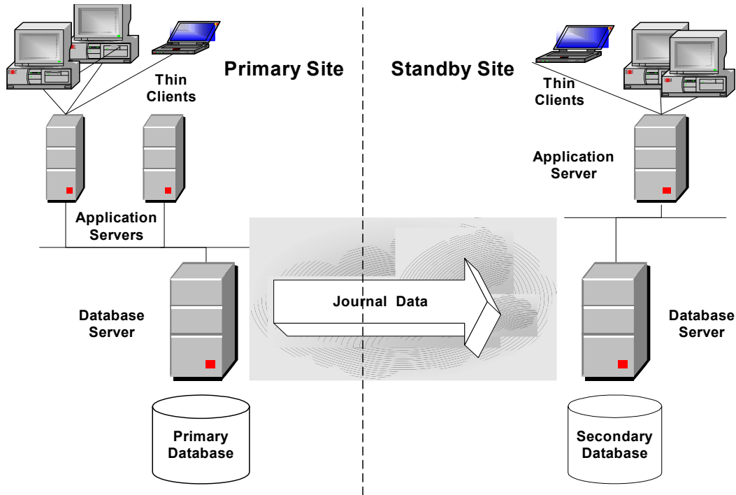
Figure 1. Overview of the JADE Synchronized Database Service
