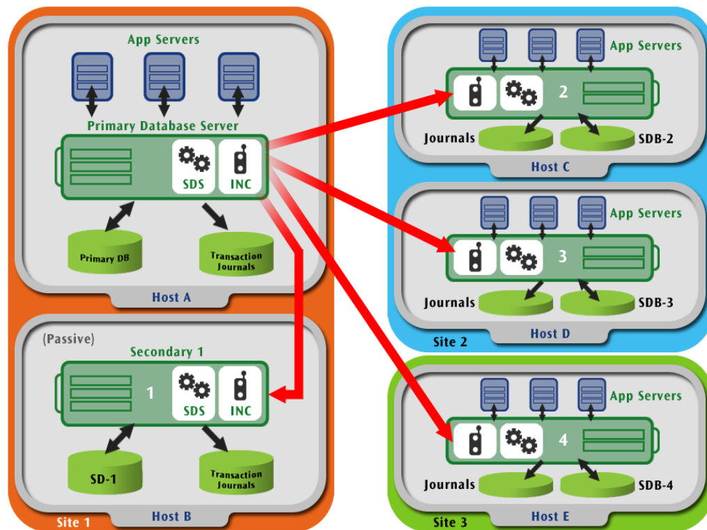
Figure 4. Hybrid Multiple Secondary Configuration
