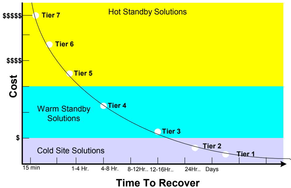
Figure 5. Tier Classification for Disaster Recovery Solutions Based on IBM SHARE Definitions
