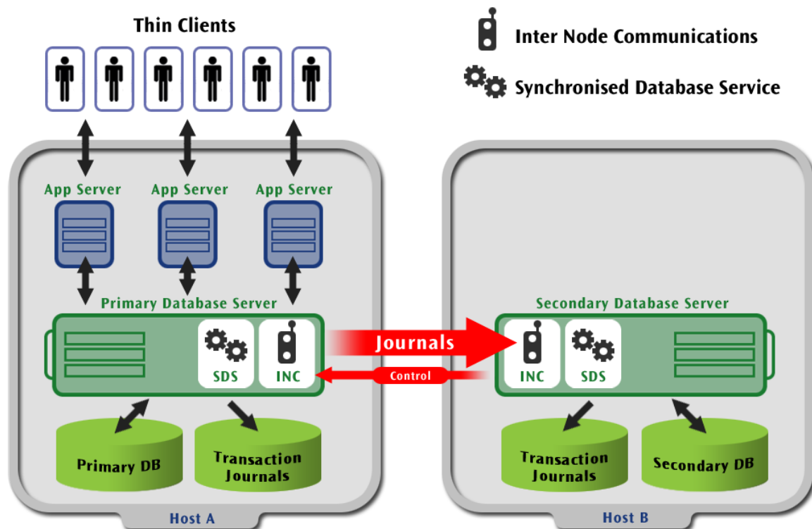
Figure 2. Passive Hot-Standby Configuration
